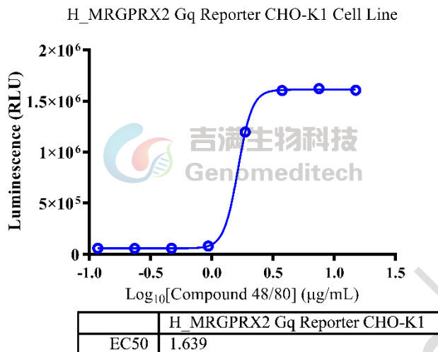
Figure 3 | Response to Compound 48/80. The H_MRGPXR2 Gq Reporter CHO-K1 Cell Line (Cat. GM-C44540) at a concentration of 1E4 cells/well (96-well format) was stimulated with serial dilutions of Compound 48/80 (MCE/HY-115768) in assay buffer (F12K + 1% FBS + 1% P.S) for 6 hours. The firefly luciferase activity was measured using the Luciferase Reporter Assay Kit (Genomeditech). The maximum induction fold was approximately [23.9]. Data are shown by drug mass concentration.
